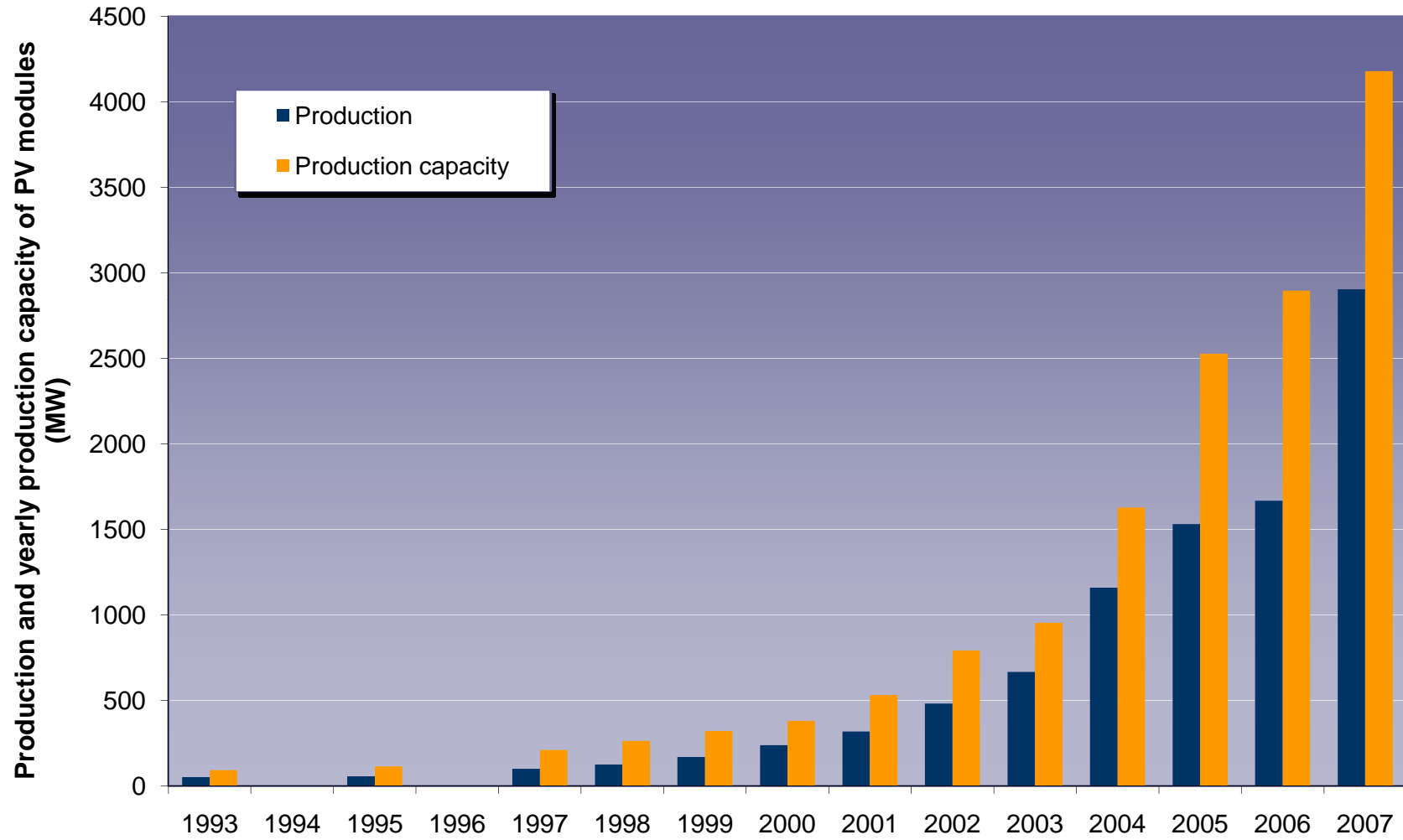
Figure 7 PV module production and yearly module production capacity in the reporting countries (MW). Years 1993-2007
