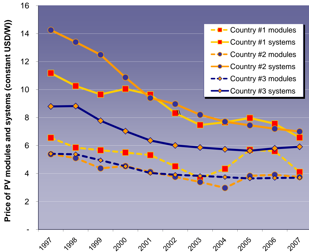
Figure 10 Evolution of price of PV modules and small-scale systems in selected reporting countries accounting for inflation effects - Years 1997-2007
