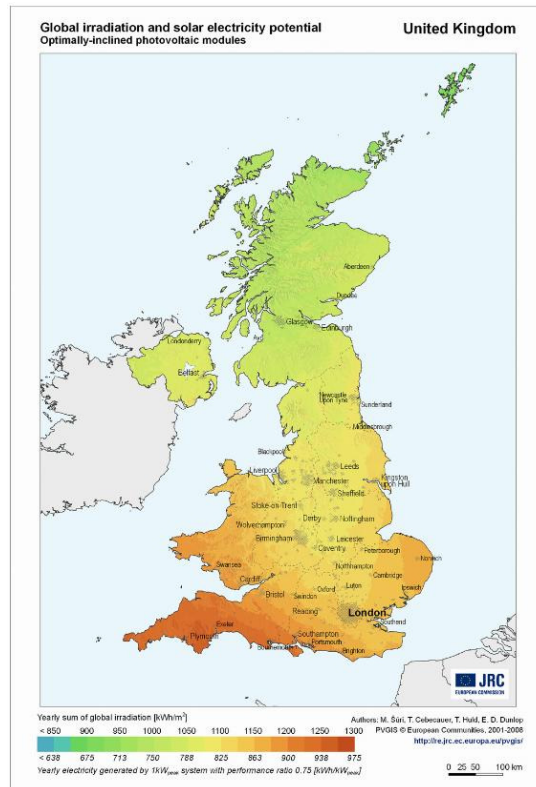
Figure 2: Solar Electricity Potential
